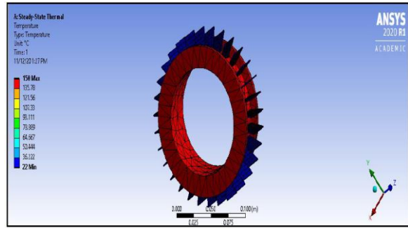
Figure 14: Temperature Distribution Over the Surface
