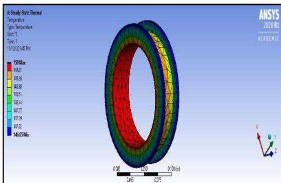
Figure 17: Temperature Distribution Over the Surface (Without Fin)
