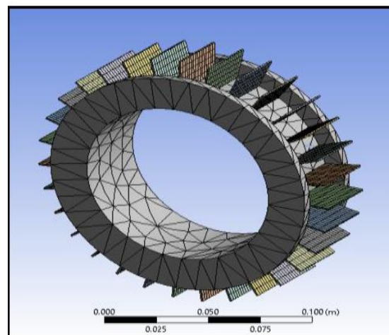
Figure 8: Meshed Model of Hub with Fins
