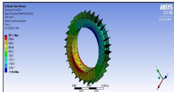
Figure 16: Directional Heat Flux Distribution Over the Surface
