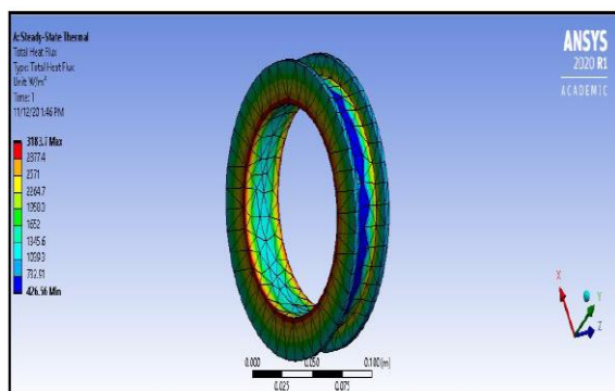
Figure 18: Heat Flux Distribution (Without Fin)
