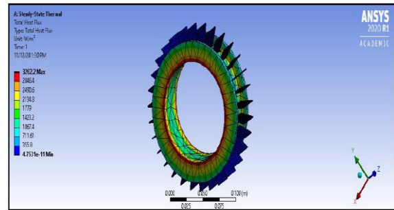
Figure 15: Heat Flux Distribution
